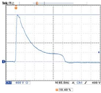
PULSE OUT connector waveform: 50Ω
