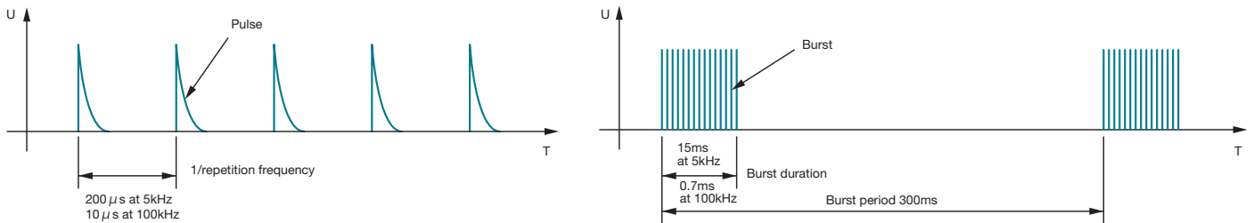
Pulse wave shape into a 50 Ω load and general graph of a fast transient/burst
