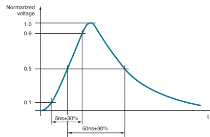
Waveshape of a single pulse into a 50 Ω load
