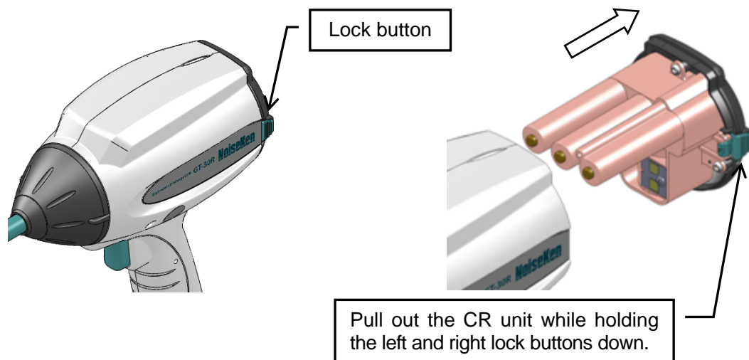
Figure 11.4 Relacing CR Unit
