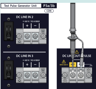
Connect to oscilloscope channel 1
